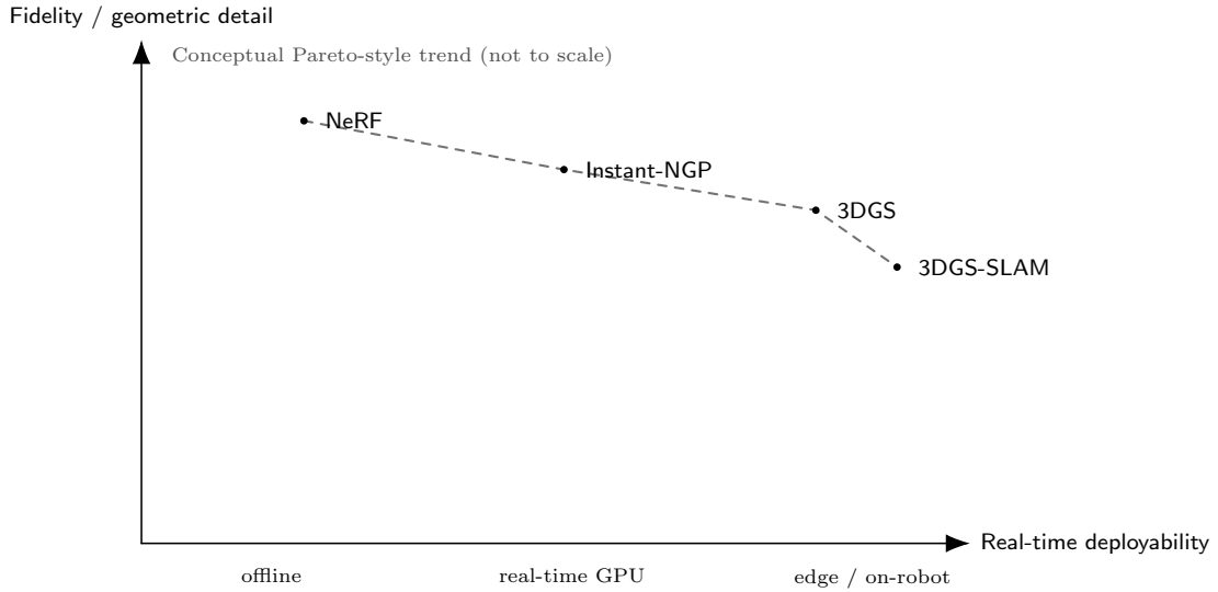
Figure 2.2: Speed-quality Pareto frontier for representative neural rendering methods.
